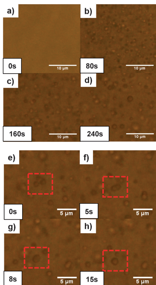
Figure 5. Bright-field optical microscopy images recorded at different times showing a–d) the transition from fragmented states (unimers) to vesicles (scale bar = 10 \mu\text{m} ), and e–h) the fusion process of two independent vesicles to form a larger vesicle. Conditions: polymer (1.5 wt %), \text{HNO}_3 (0.7 M), \text{NaBrO}_3 (0.2 M), and MA (0.025 M) at 26 ^\circ\text{C} .
